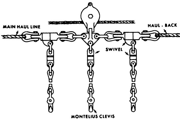
2 BUTT RIGGING FOR A TIGHT-LINING SYSTEM
